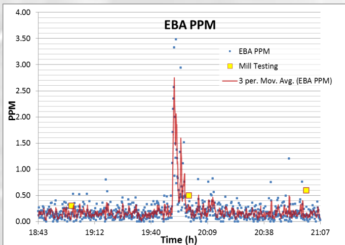
ODI detected a dirt outbreak not observed by the hourly mill testing
